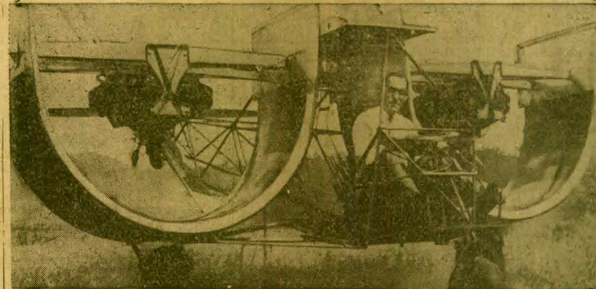
NOW HERE'S SOMETHING A LITTLE DIFFERENT . . . This is the Custer channel wing plane, invented by Willard R. Custer and being tested by the National Aircraft corporation of Hagerstown, Md. Believe it or not, the ship has flown several times. The plane, with its elliptical wings, is controlled entirely by the action of its engine. It has no ailerons, flaps or brakes and no wing area except the channels which have a diameter of six feet. Gross weight of the plane is approximately 1,000 pounds, and the total wing area, including the space between the channels, is 42 square feet. No, it isn't a helicopter; it's a plain plane with elliptical wings.
